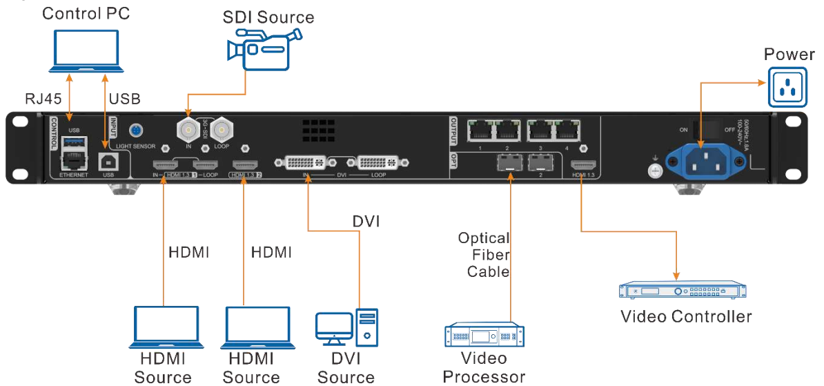
Figure 5-33 HDMI output
